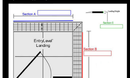
Two Sided Entry-Level Landing (Left Side Approach)
